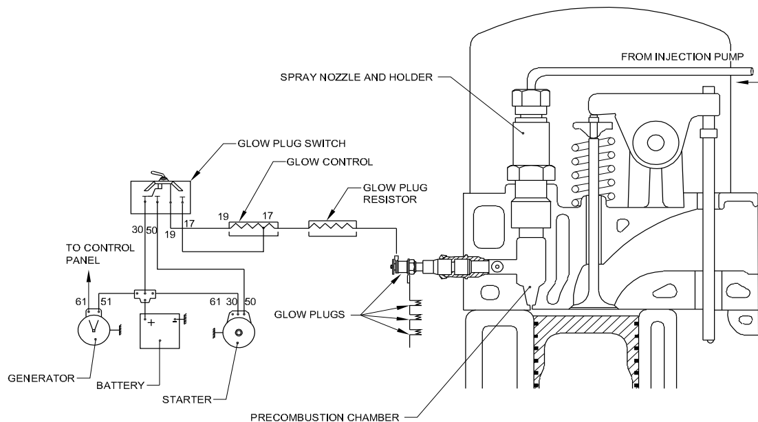
IGNITION CIRCUIT DIAGRAM OF GLOW PLUG SYSTEM IN A DIESEL ENGINE
