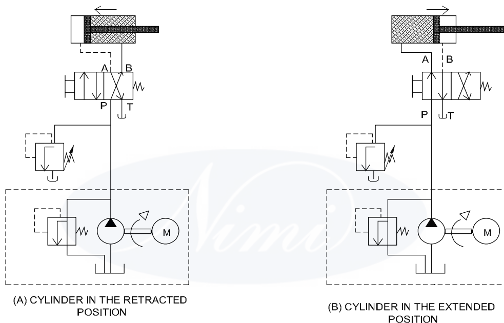
Figure 8: Two positions of the circuit for the control of a double - acting hydraulic cylinder
