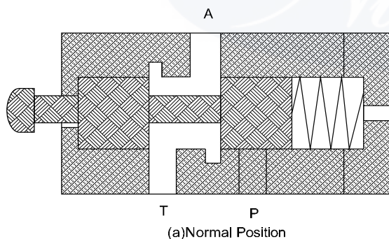
Figure 5: Cross-sectional views of a spool type 3/2-DC hydraulic valve (NC type) in its normal and actuated positions
