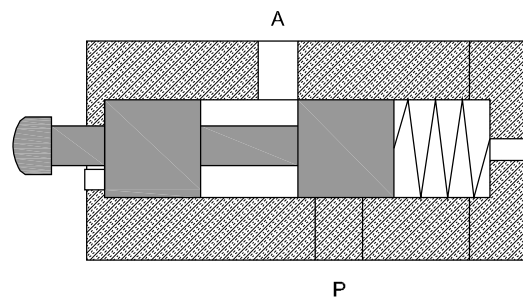
Fig 4(a) Normal position
