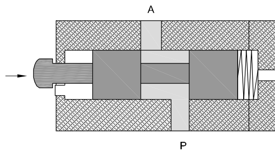
Fig 4 (b) Actuated position
