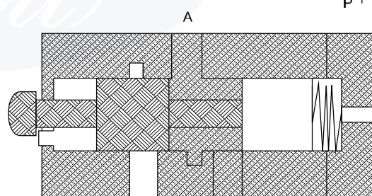
(b)Actuated Position
