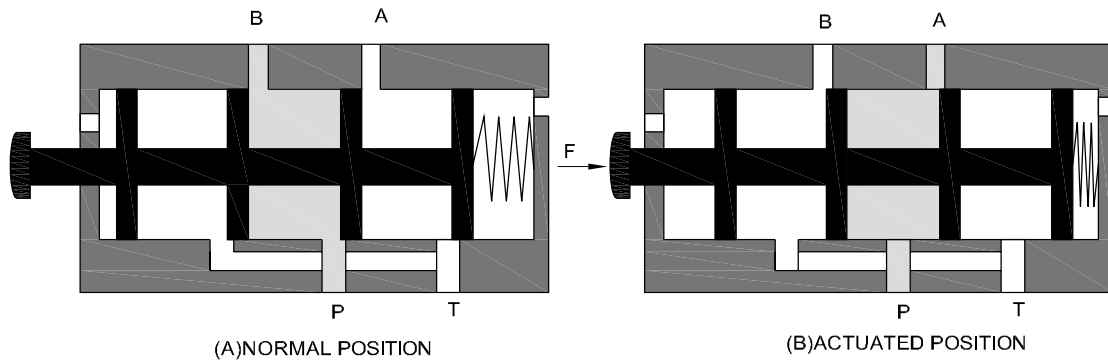
Figure 7: Cross sectional views of a manually actuated 4/2 DC hydraulic valve in its normal and actuated position
